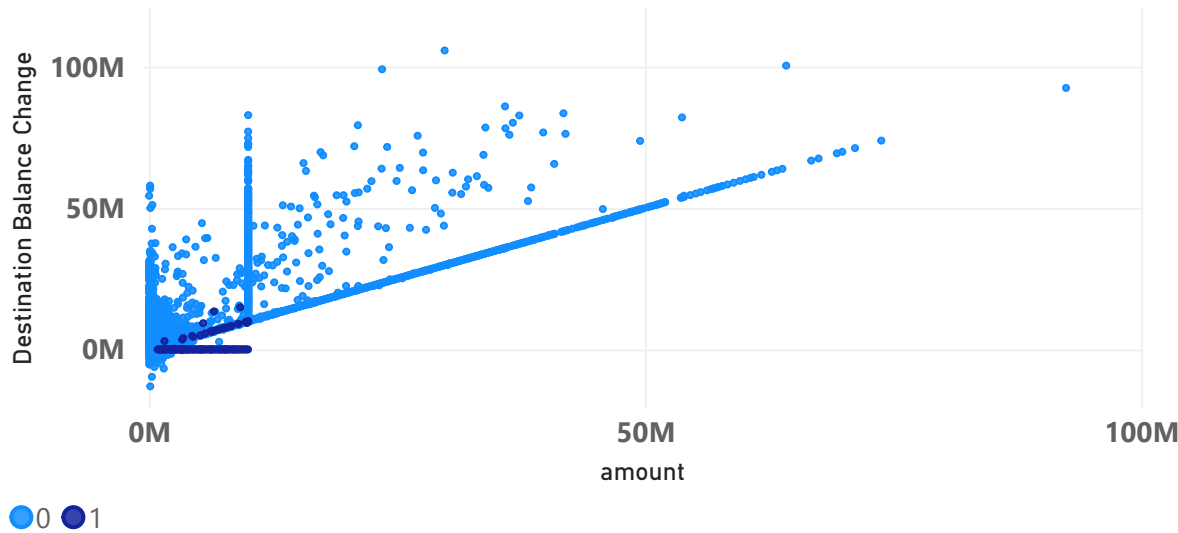
Amount Vs Destination Balance Change
